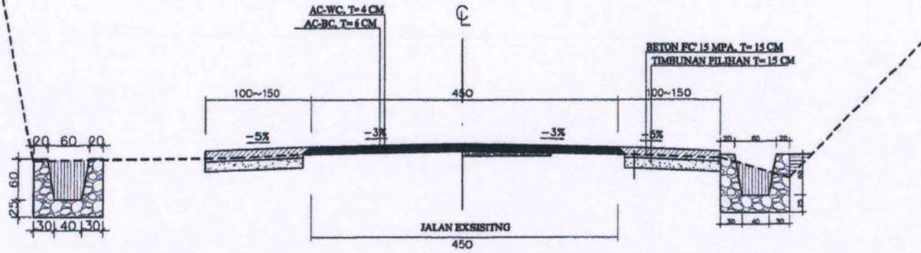
TYPICAL JALAN (STA 156+280 S/D 156+355)
