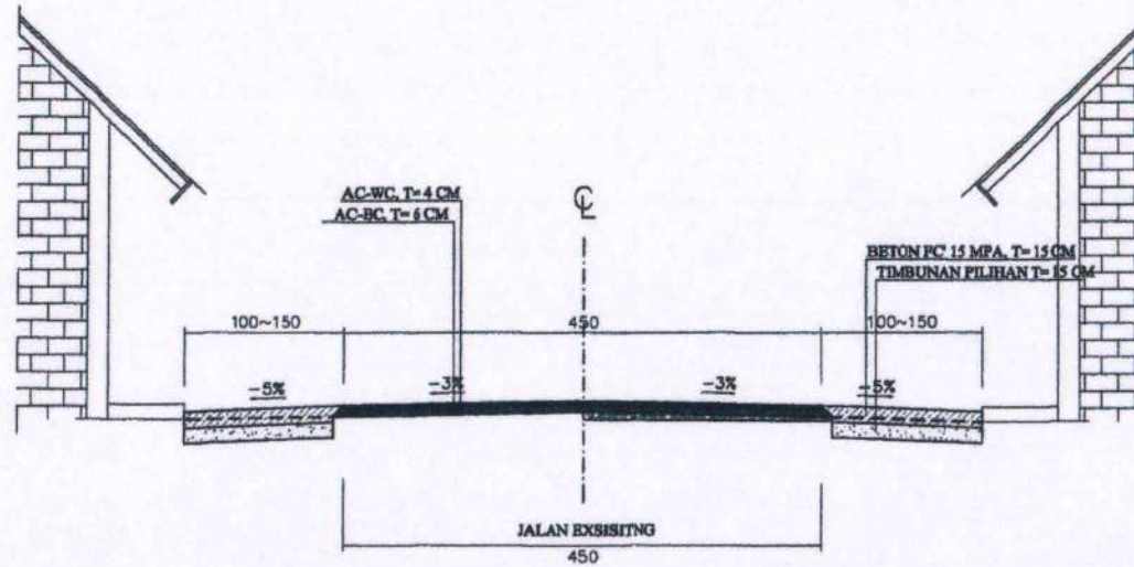
TYPICAL JALAN (STA 157+180 S/D 157+380)
