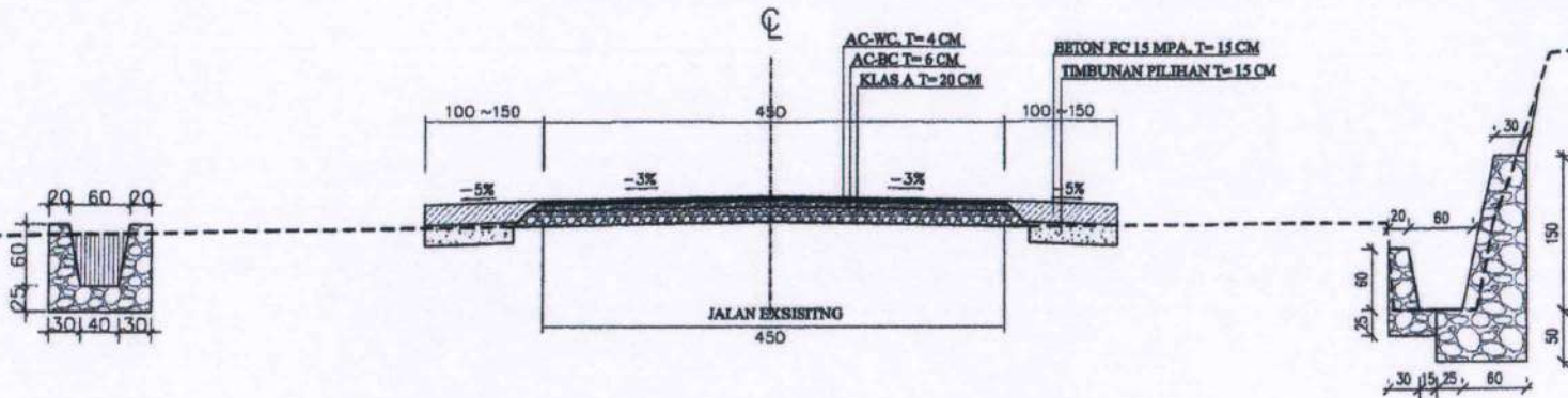
TYPICAL JALAN (STA 156+750 S/D 157+000)
