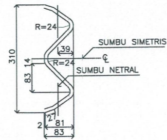
ENLARGED POTONGAN A-A ( SIMILAR POTONGAN B-B ) SKALA 1:5
