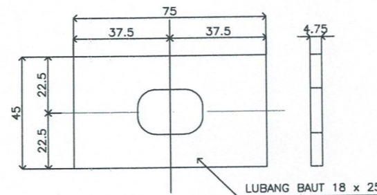
RECTANGULAR WASHER
