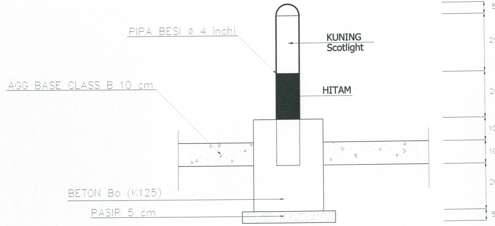
TAMPAK SAMPING
