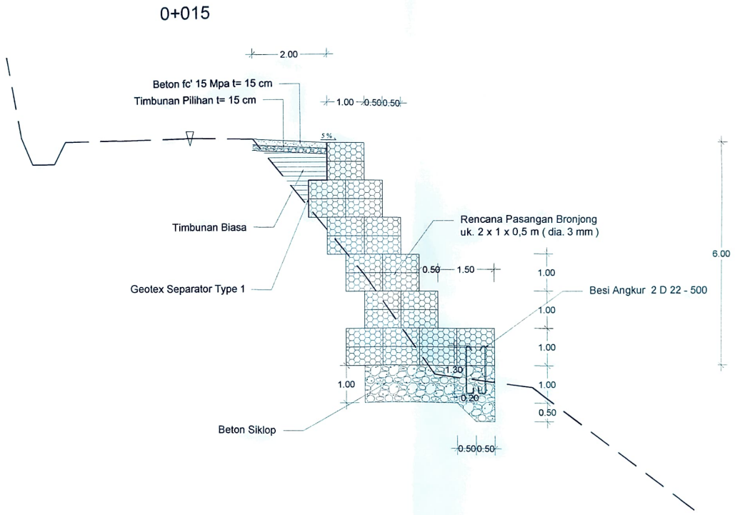
POTONGAN A - A Scale 1 : 75
