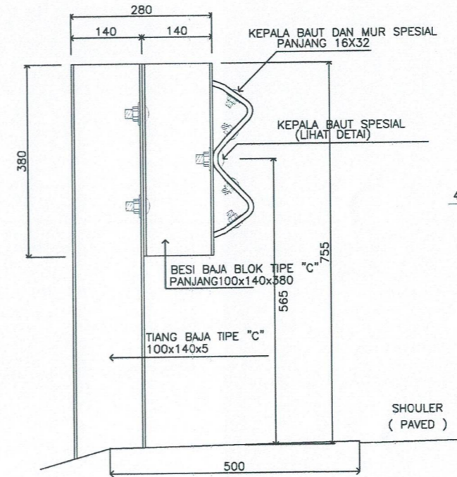
RAIL OFFSET ( DETAIL-C )
