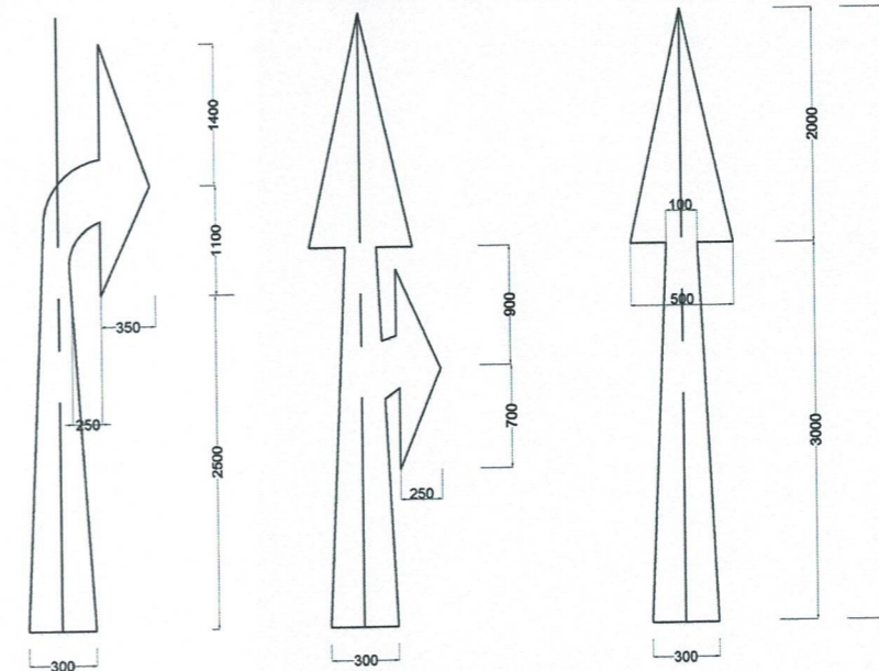
STANDAR PANAH RM-8
